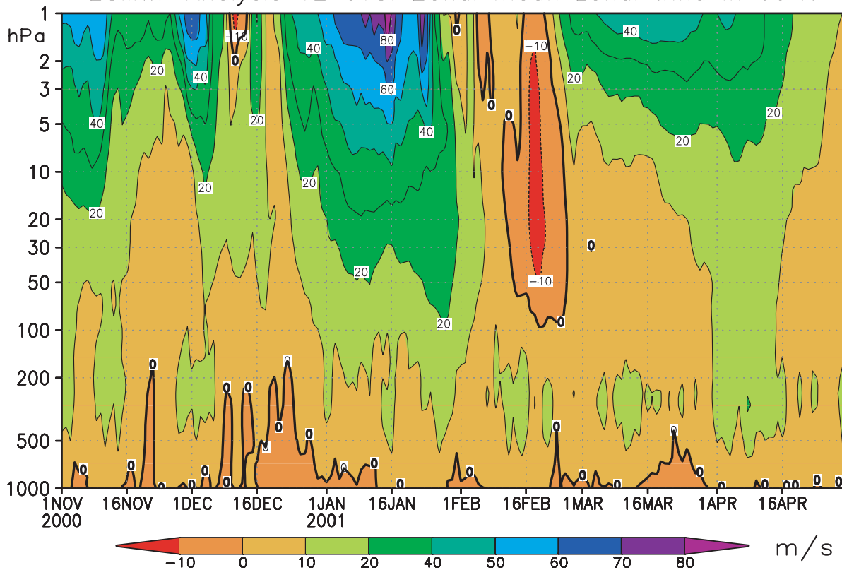
Figure 1: Time-height sections of North Pole temperature (upper panel) and of zonal mean zonal wind at 60°N (lower panel) during the winter 2000/01 derived from the ECMWF analyses. [Courtesy of B. Naujokat, FU Berlin].
