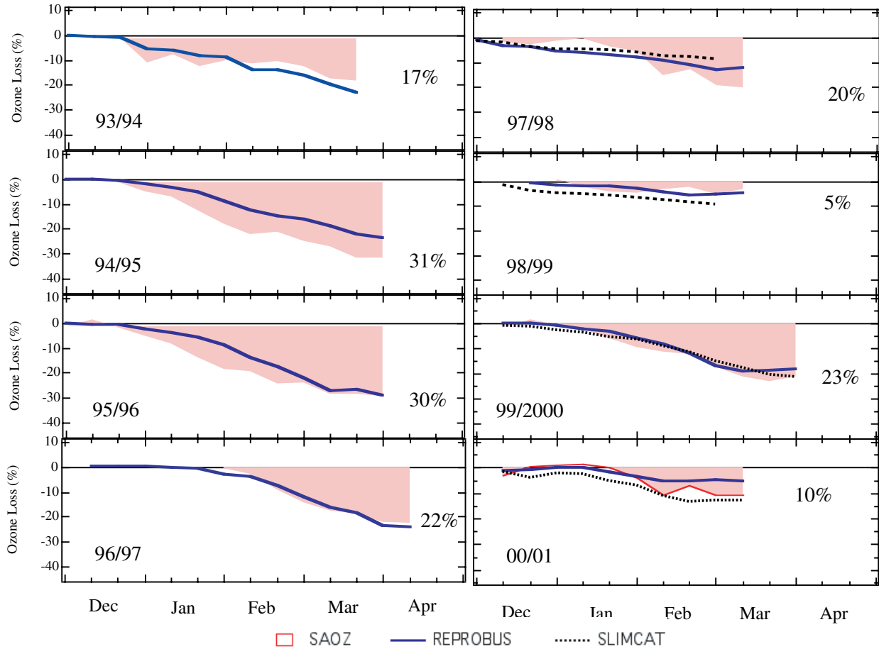
Figure 10: Chemical depletion of total ozone in the Arctic vortex deduced from (i) comparing SAOZ measurements with the Reprobus passive ozone (red hatched area); (ii) the Reprobus CTM (blue line); and (iii) the SLIMCAT CTM. (Courtesy of F. Goutail, CNRS-SA)
