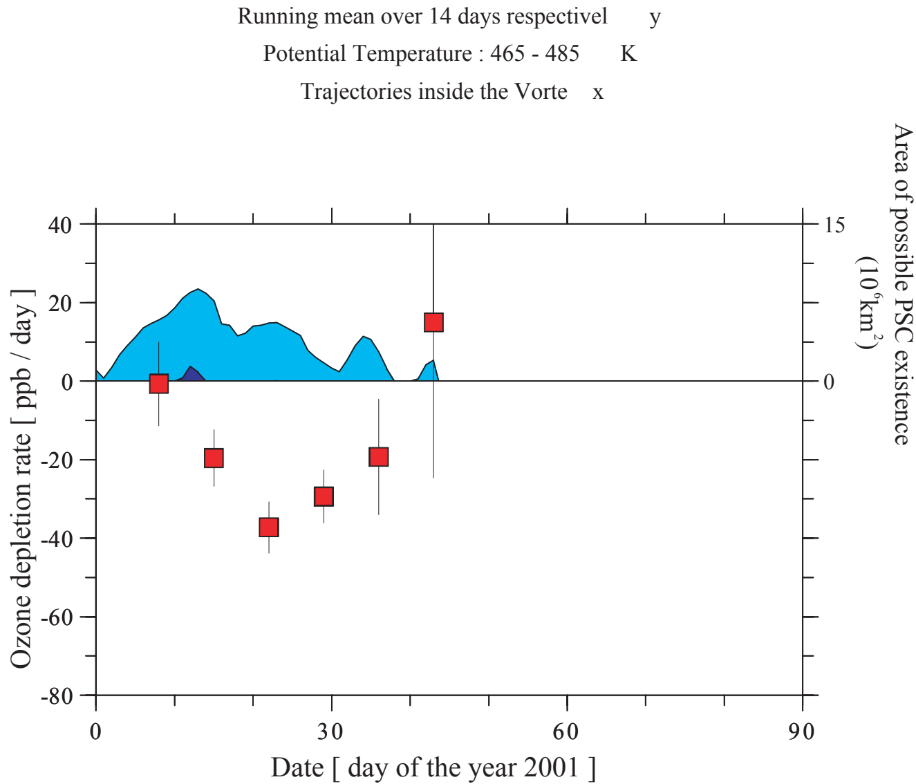
Figure 9: Ozone loss rates (ppbv/day) at 475K (about 18km altitude) are shown as a function of day of year in the lower panel. The blue hatched area in the upper panel indicates the area where temperatures are below the NAT existence temperature. The purple hatched area in the upper panel indicates the area where temperatures are below the ice existence temperature. (Courtesy of M. Rex, AWI-Potsdam)
